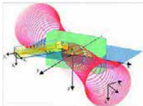
Fig. 4.24: A graphical representation of a typical confocal micro-PIXE geometry. A rectangular ion micro-beam (yellow) irradiates a sample (green object), which is observed through the sensitive detection-volume of a polycapillary lens (the red surface represents an iso-surface of the lens acceptance for a given X-ray energy). (Reproduced from D. Sokaras et al., J. Anal. At. Spectrom. , 2009, 24 , 611.)
