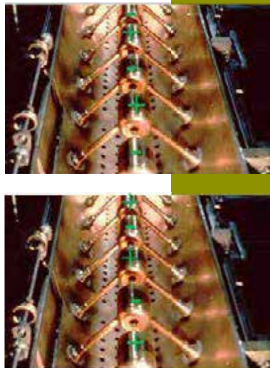
Fig. 2.2: The electrodes in one type of linear accelerator at two different times, showing how acceleration is achieved.
