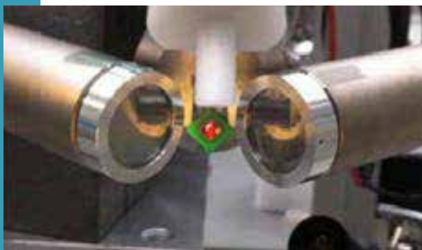
Fig. 4.19: A view of the LABEC external beam PIXE set-up for atmospheric aerosol studies, with the low-energy X-ray detector (upper part of the picture, showing also a magnetic proton deflector assembly), the high-energy X-ray detectors (on the left and the right), the silicon-nitride beam extraction window (in the centre of the figure), and the micro-camera (in the low right corner). Laboratorio di Tecniche Nucleari per l'Ambiente e i Beni Culturali (LABEC) is the 3-MV Tandatron accelerator of the Istituto Nazionale di Fisica Nucleare (INFN) in Florence. (Reproduced from G. Calzolari et al., Nucl. Instr. and Meth. B, 2015, 363 , 99.)
