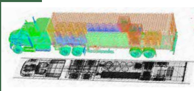
Fig. 6.3: X-ray data from Passport Systems scanning technology, which can detect a wide variety of materials.
