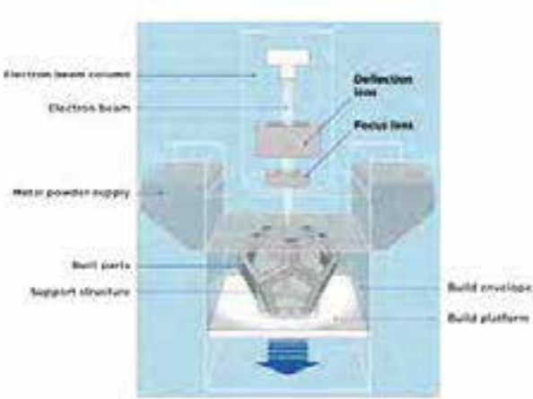
Fig. 4.9: The scheme for additively building up a 3D structure by melting successive metal powder layers using an e-beam (courtesy of Additively).
