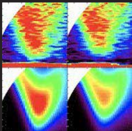
Fig. 8.1: Neutron inelastic scattering measurements can be used to investigate the exotic magnetic structures of metal compounds – here, the spinel, iron scandium sulfide ( \text{FeSc}_2\text{S}_4 ) – that throw light on physics that could lead to novel electronic devices (credit: PSI/A. Biffen et al., Phys.Rev.Lett., 2017, 118 , 067205).
