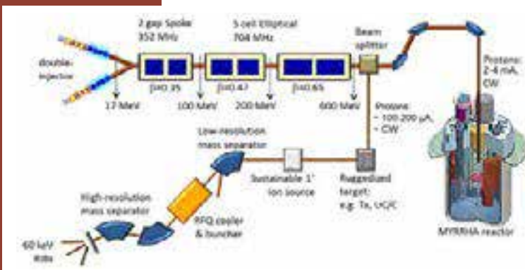
Fig. 5.4: The general layout of the MYRRHA system.
