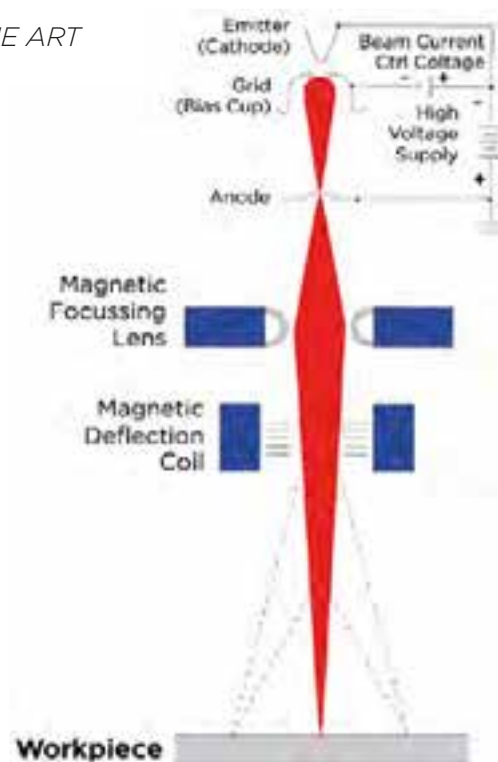
Fig. 4.1: The principle of electron-beam generation and direction for focused beam applications under vacuum conditions.
