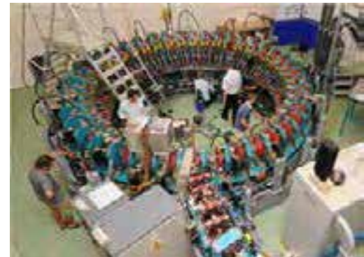
Fig. 2.8: The fixed field alternating gradient accelerator (FFAG), EMMA, built in the UK.
