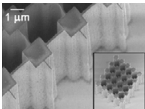
Fig. 4.25: A scanning electron microprobe image of 2-micrometre-square pillars written in a 10-micrometre-thick layer (inset). Linking the pillars are high-aspect-ratio walls of widths 60 and 120 nanometres. The structures were written with a 1-MeV proton beam. (Reproduced from J. A. van Kan et al., Appl. Phys. Lett., 2003, 83 , 1629.)
