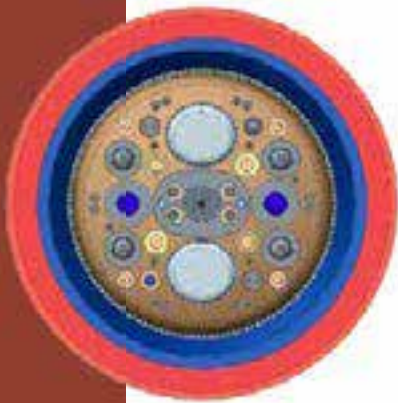
Fig. 5.2: The layout of the MYRRHA reactor vessel.
