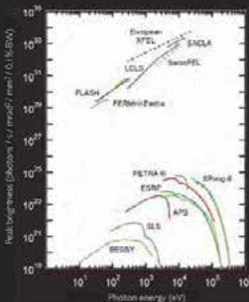
Fig. 7.8: The photon energy and brightness relationship for a number of photon sources.
