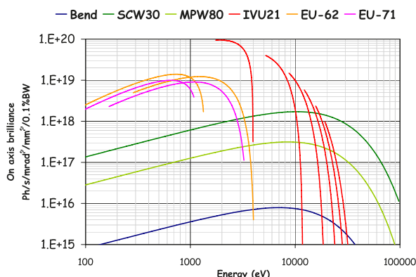
Fig. 7.9: The brilliance dependence on wavelength for a third-generation SR (ALBA) for different insertion devices, as well as the conventional dipole magnets that bend the electron beam around the synchrotron (blue).
