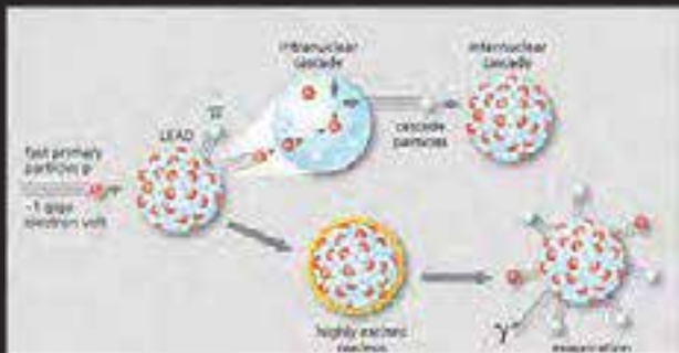
Fig. 8.3: In the spallation process, neutrons are emitted following the bombardment of heavy nuclei with highly energetic particles.
