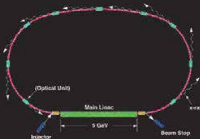
Fig. 7.7: A schematic of the principle of the energy recovery linac (credit: Cornell University).
