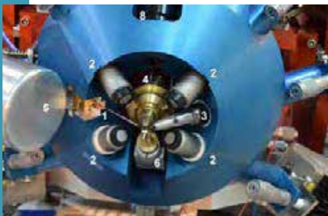
Fig. 4.21: A view of the AGLAE external microprobe used to study artefacts at the Louvre Museum. 1: IBIL collection optical fibre, 2: high energy X-ray detectors, 3: low energy X-ray detector, 4: annular charge particle detector, 5: gamma-ray detector, 6: dose detector for normalisation, 7: silicon-nitride beam extraction window, 8: video-microscope. Accélérateur Grand Louvre d'analyse élémentaire (AGLAE) is the 2 MV Pelletron accelerator of the Centre de Recherche et de Restauration des Musées de France (C2RMF) based at the Louvre. (Reproduced from L. Pichon et al., Nucl. Instr. and Meth. B, 2015, 348 , 68.)
