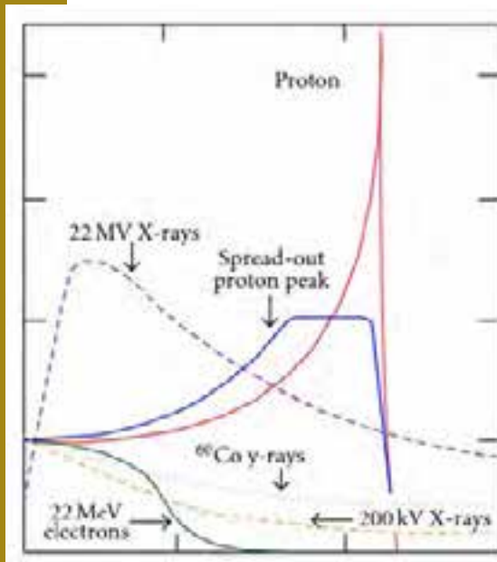
Fig. 3.5: The relative dose as a function of depth for X-rays (photons), electrons and protons in water. A proton beam at a fixed energy produces the red curve, ending in the so-called Bragg peak. This can be spread out over the tumour volume by overlapping the dose created from multiple beams with different proton energies and fluence, the sum of which is called the spread-out Bragg peak (SOBP) (credit: M. Cianchetti, Int. J. Otolaryngology, 2012, 3, 325891, CC BY 3.0.)
