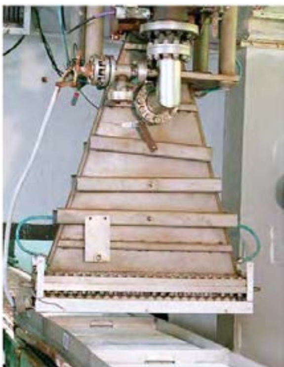
Fig. 4.12: E-beam technology for sterilising medical products.
